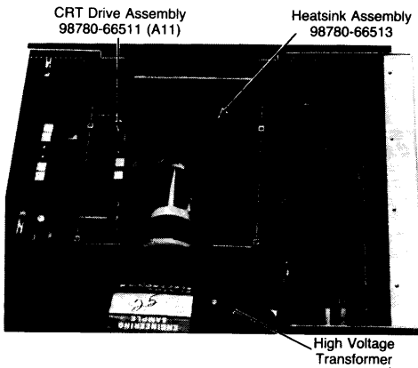
Assemblies in High Voltage Cage
